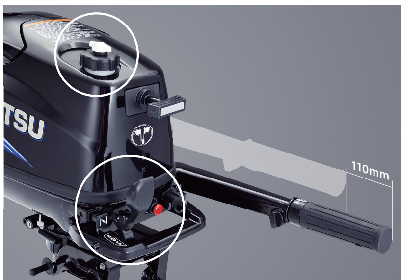
FRONT SHIFT LEVER / LONGER TILLER HANDLE / FUEL TANK CAP
